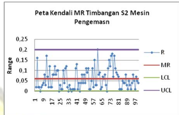
Gambar 5 Peta Kendali MR Timbangan S2
