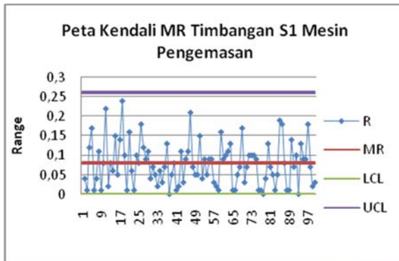
Gambar 4 Peta Kendali MR Timbangan S1
