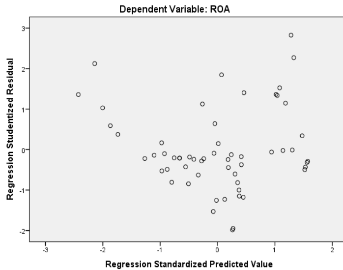
Scatterplot
