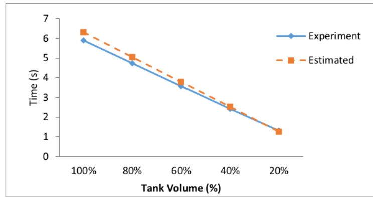
Figure 3. The Comparison Pump Test
