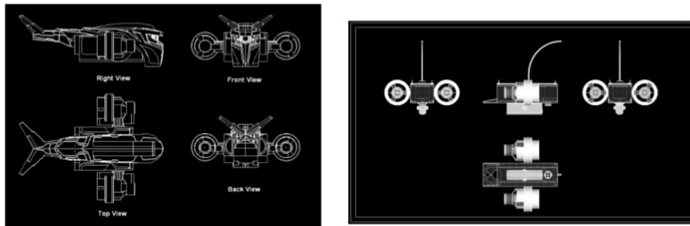
Figure 1. Component Design of the ROV
