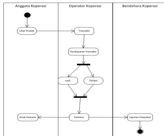
Gambar 4. Activity Sistem Berjalan Sumber: Activity Prosedur Sistem Usulan (2021)
