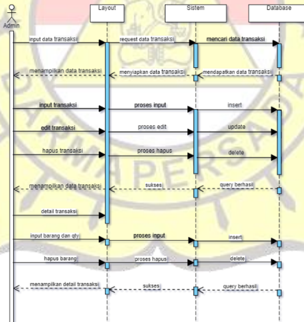
Gambar 4. Sequence Diagram Transaksi
