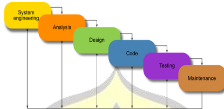
Gambar 1. Metode Waterfall
