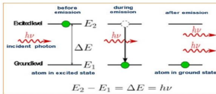
Gambar 3 Prinsip Kerja Laser Diode
