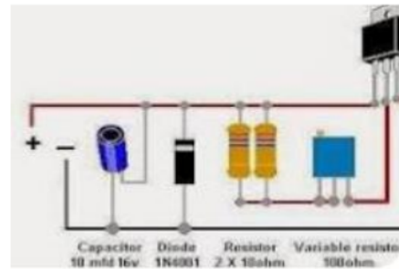
Gambar 5 Rangkaian Laser Dioda
