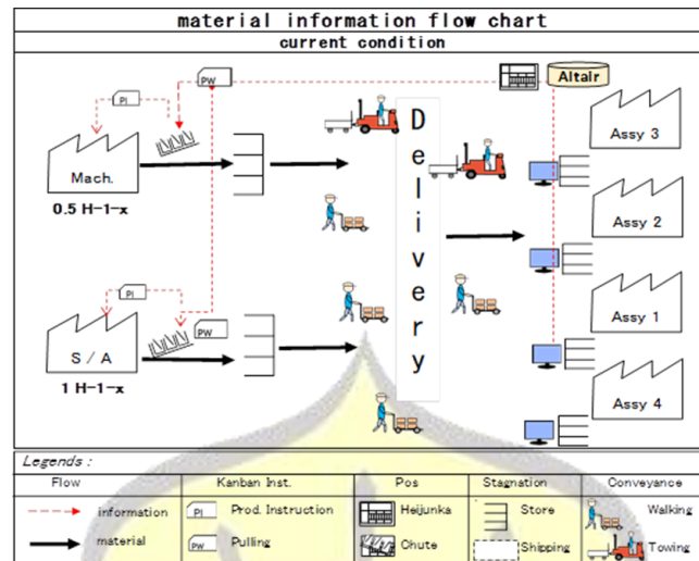
Gambar 4. MIFC Penanganan Manual Transfer Material
