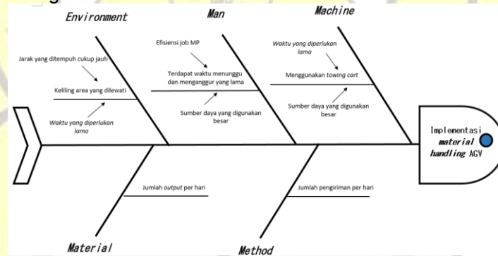
Gambar 5. Fishbone Diagram
