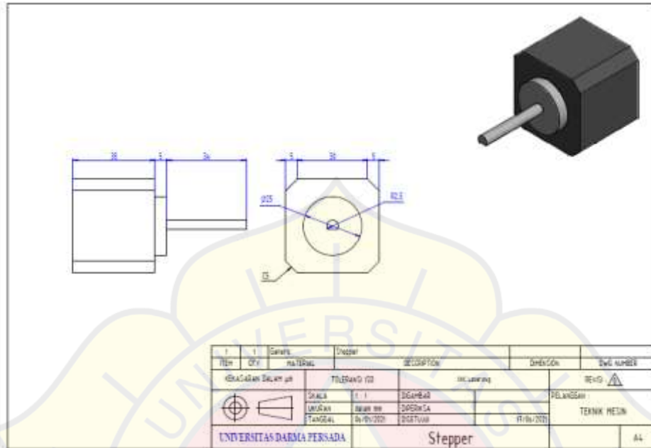
Gambar 3. 9 Motor Stepper
