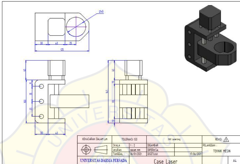
Gambar 3. 7 Case Laser
