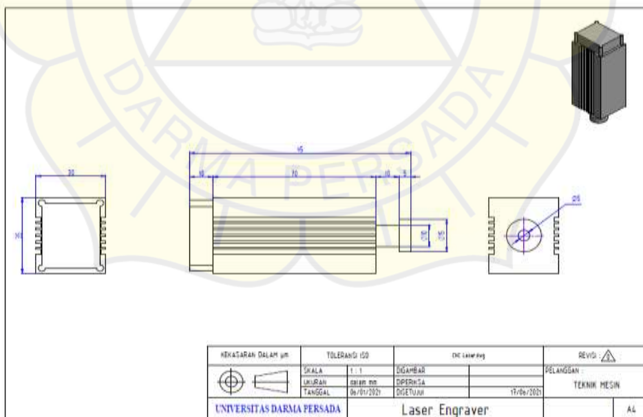
Gambar 3. 6 Laser Engraving
