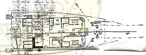
FORECASTLE DECK
