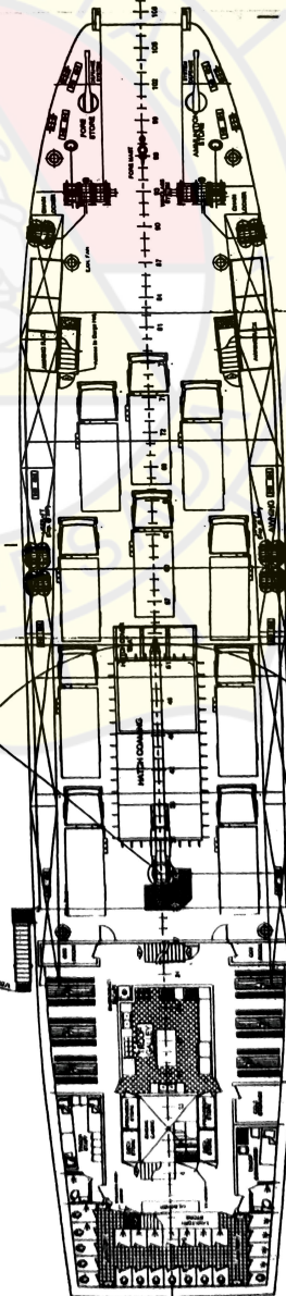
MAIN DECK
