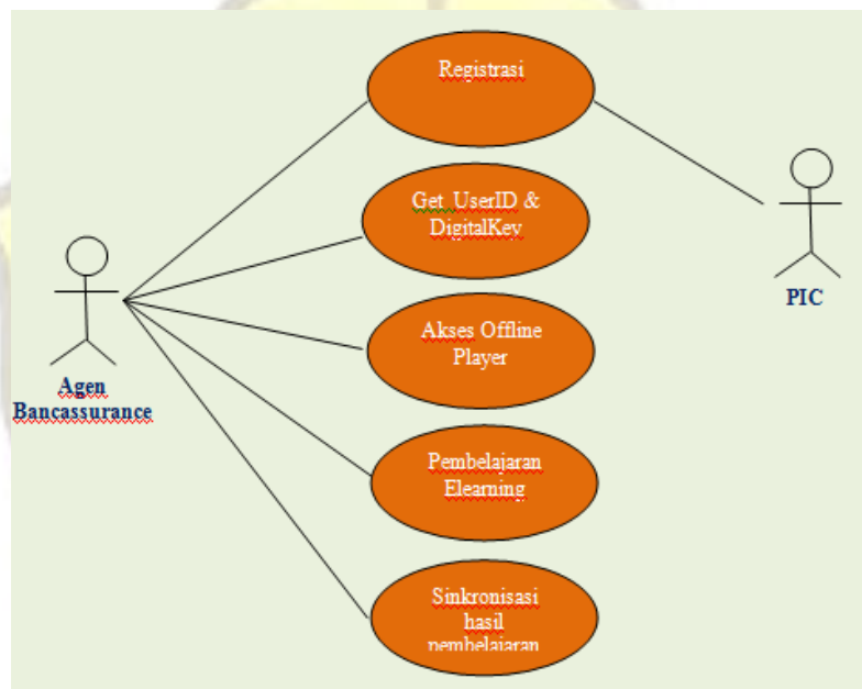
Gambar 6. Use case sistem offline player
