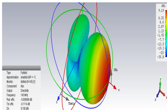
Fig.9. Radiation Pattern at 145 Mhz Frequency Simulation Result
