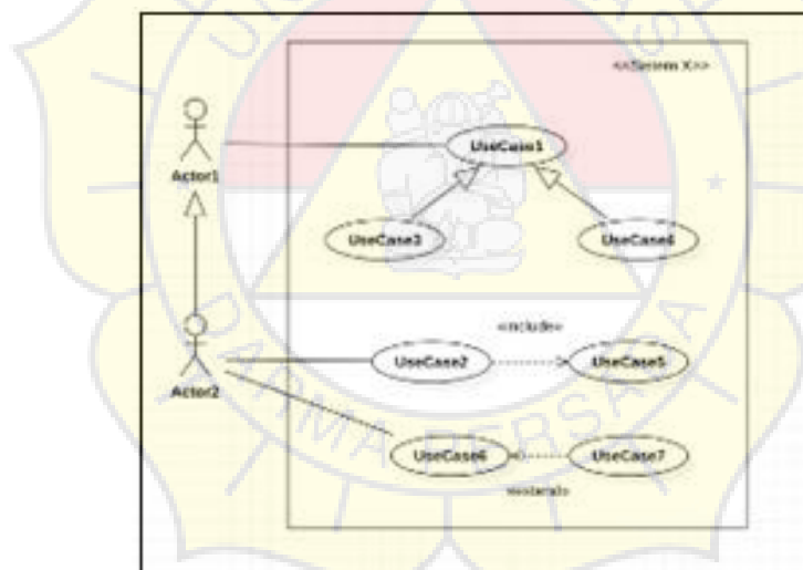
Gambar 2. 2 Activity Diagram
