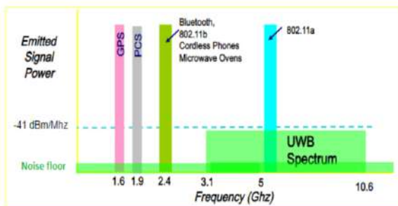
Figure 1. UWB versus other Radio Communication Systems [2]
