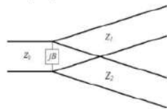
Figure 7. T-Junction Power Divider [22].
