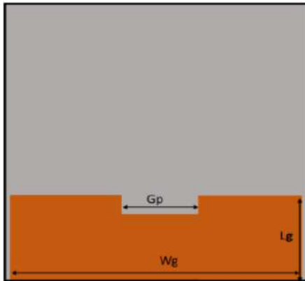
Figure 8. The ground plane's DGS.
