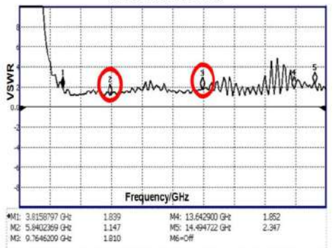
Figure 13. VSWR Versus Frequency of the simulation result.
