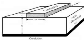
Figure 6. Microstrip line
