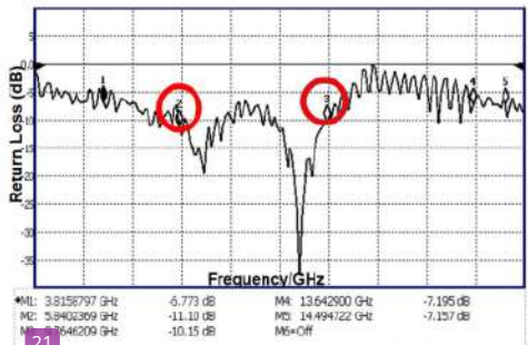
21 Figure 12. Return loss Versus Frequency of measurement result.
