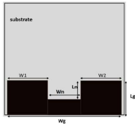
Figure 10. Design of antenna bottom view.
