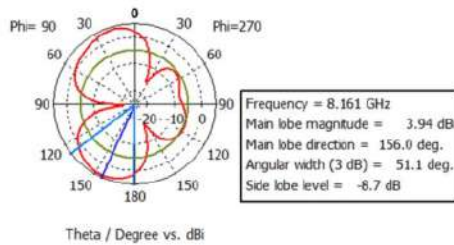
Figure 18. Far-field on the frequency of 8.161 GHz in the theta.
