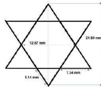
Figure 5. Star patch design
