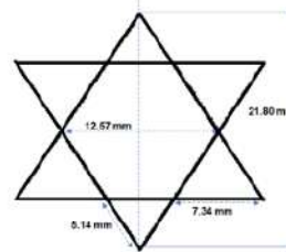
Figure 5. Star patch design.
