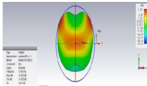
Figure 15. Radiation pattern at a frequency of 5.796 GHz
