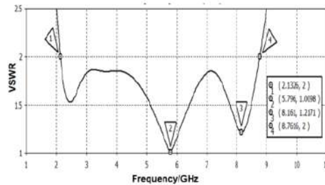
Figure 13. VSWR Versus Frequency of the simulation result.
