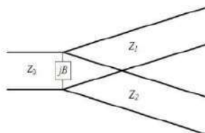
Figure 7. T-Junction Power Divider [23]
