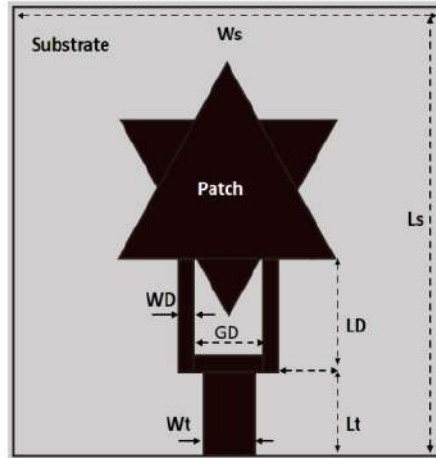
Figure 9. Design of antenna top view.
