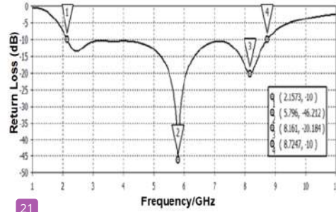
21 Figure 11. Return loss Versus Frequency of simulation result.
