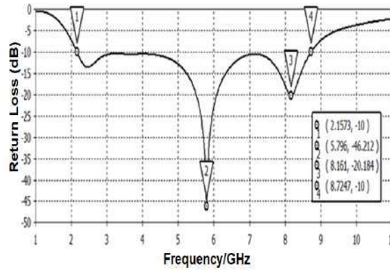
Figure 11. Return loss Versus Frequency of simulation result.
