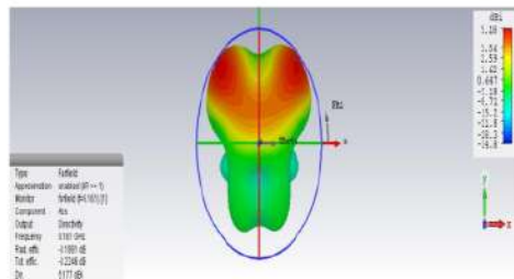
Figure 16. Radiation pattern at a frequency of 8.161 GHz
