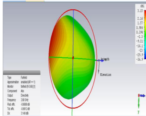
Farfield Directivity Abs (Azimuth=90)
