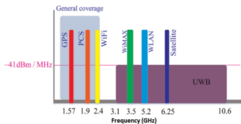
Gambar 1. Spektrum Ultra-Wideband .
