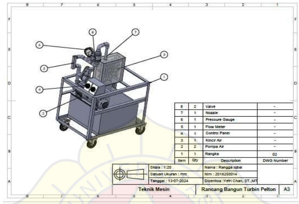
Gambar 5.5 Turbin pelton
