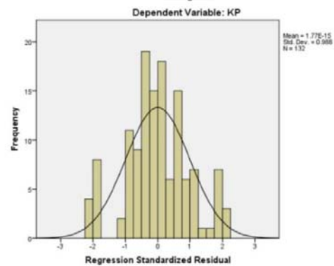
Histogram
