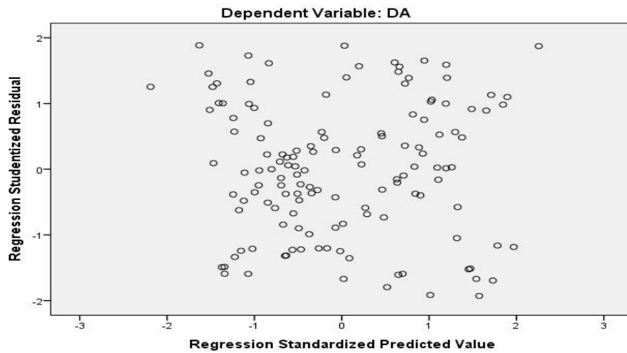
Scatterplot
